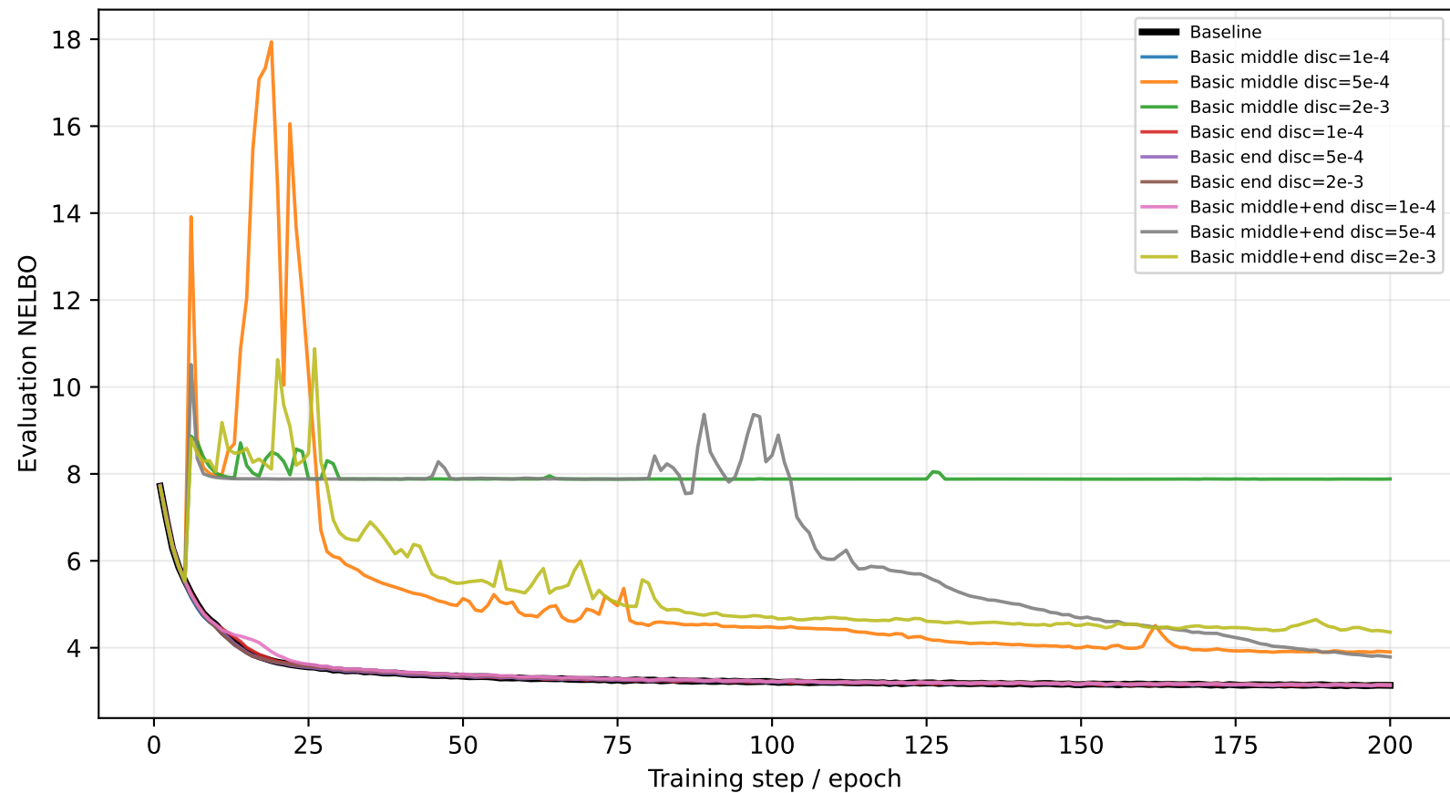
Basic Discriminator Guidance: Evaluation NELBO
