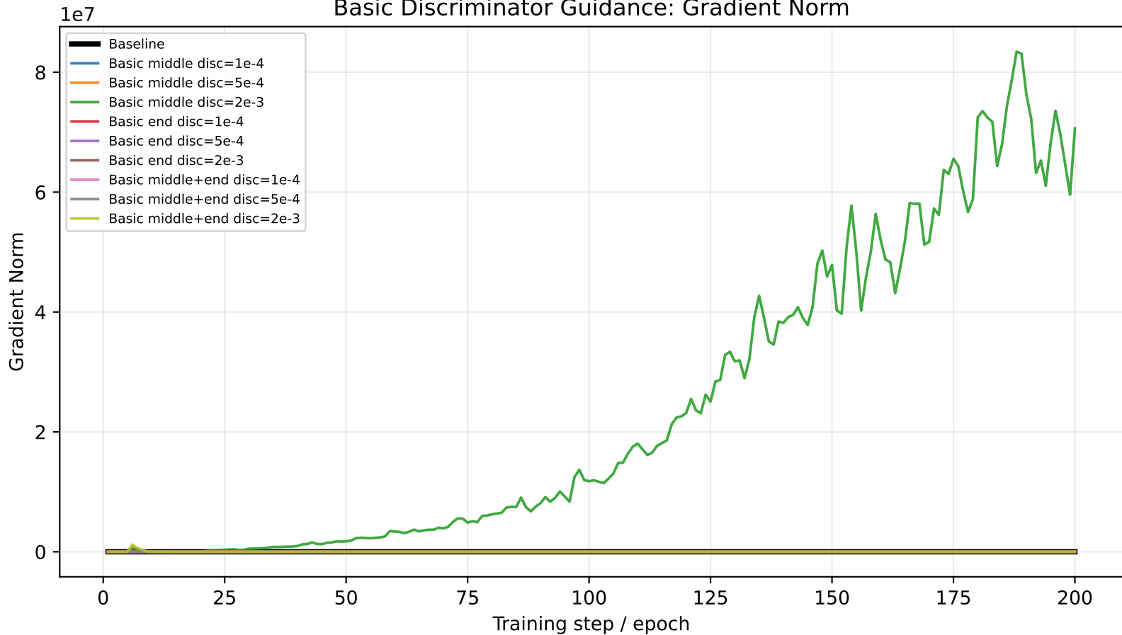
Basic Discriminator Guidance: Gradient Norm
