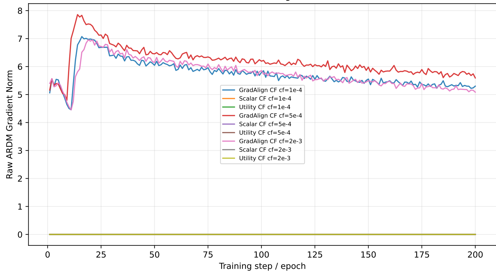
Counterfactual Feature-Credit Guidance Diagnostic: Raw ARDM Gradient Norm
