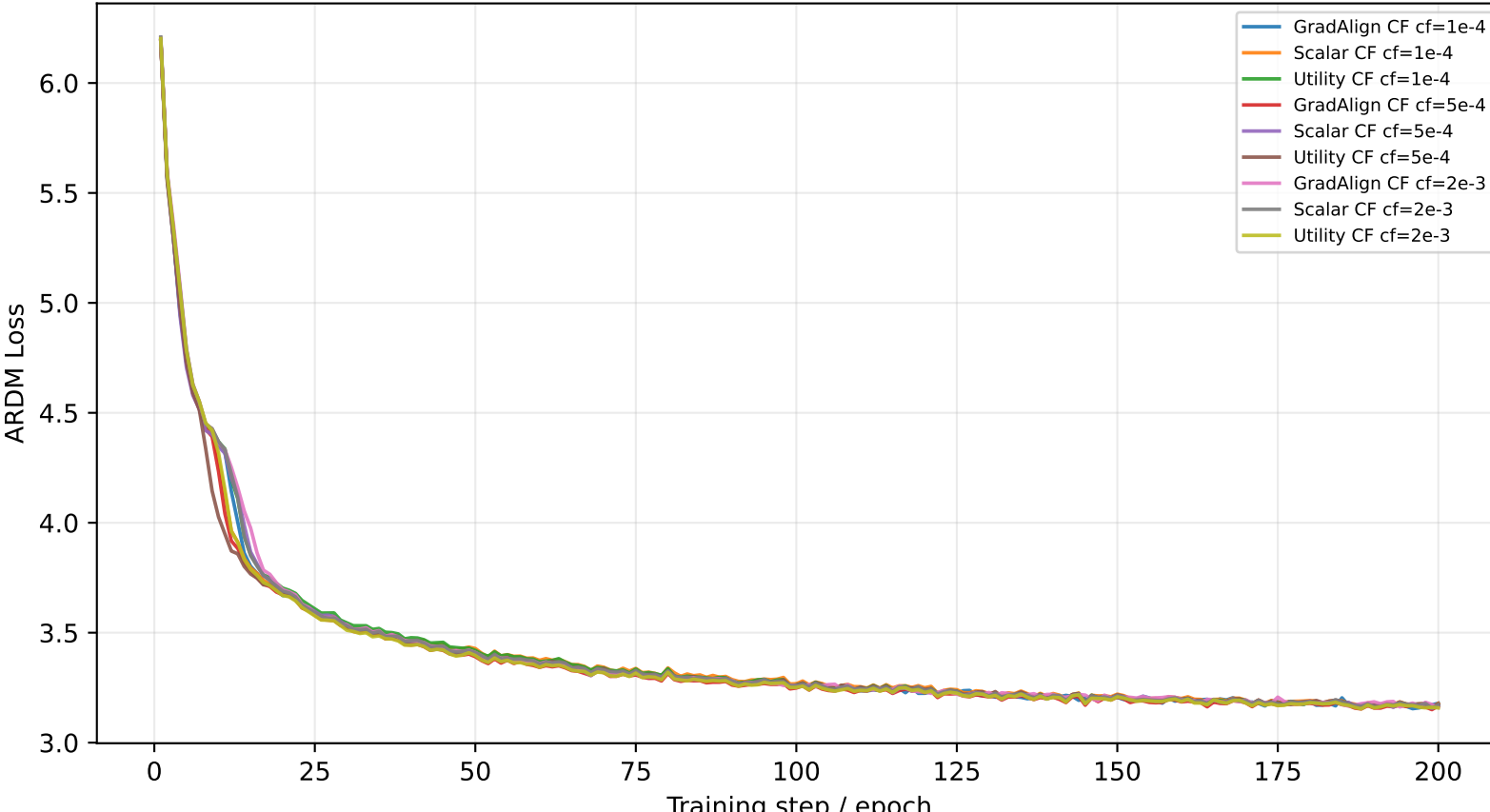
Counterfactual Feature-Credit Guidance Diagnostic: ARDM Loss
