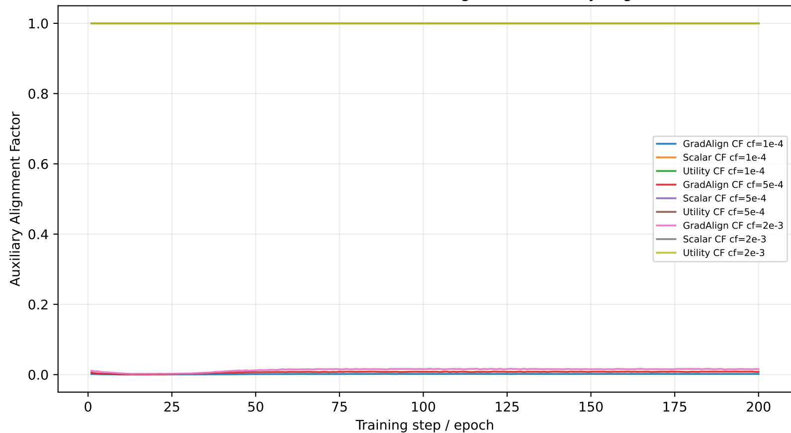
Counterfactual Feature-Credit Guidance Diagnostic: Auxiliary Alignment Factor
