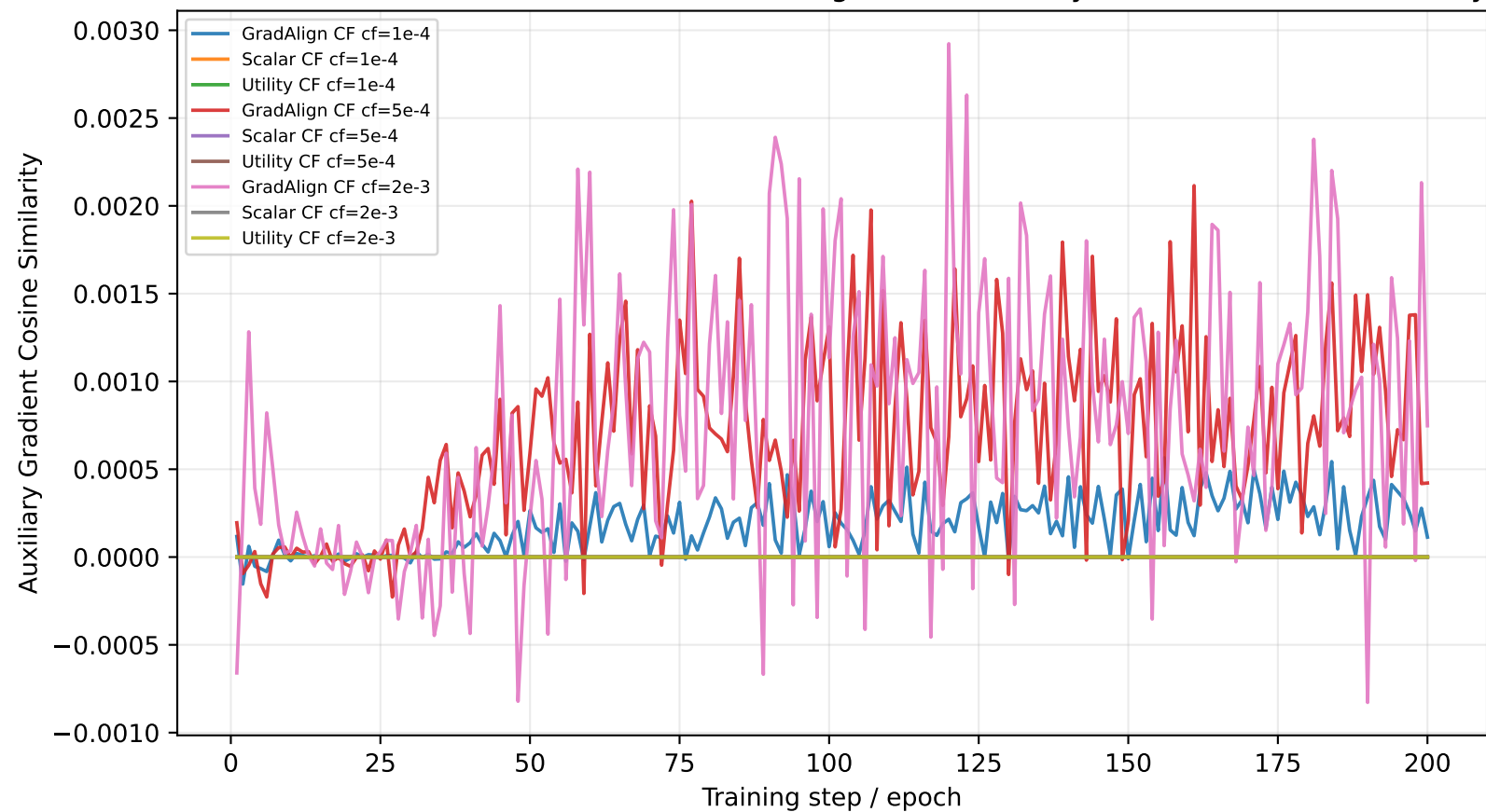
Counterfactual Feature-Credit Guidance Diagnostic: Auxiliary Gradient Cosine Similarity
