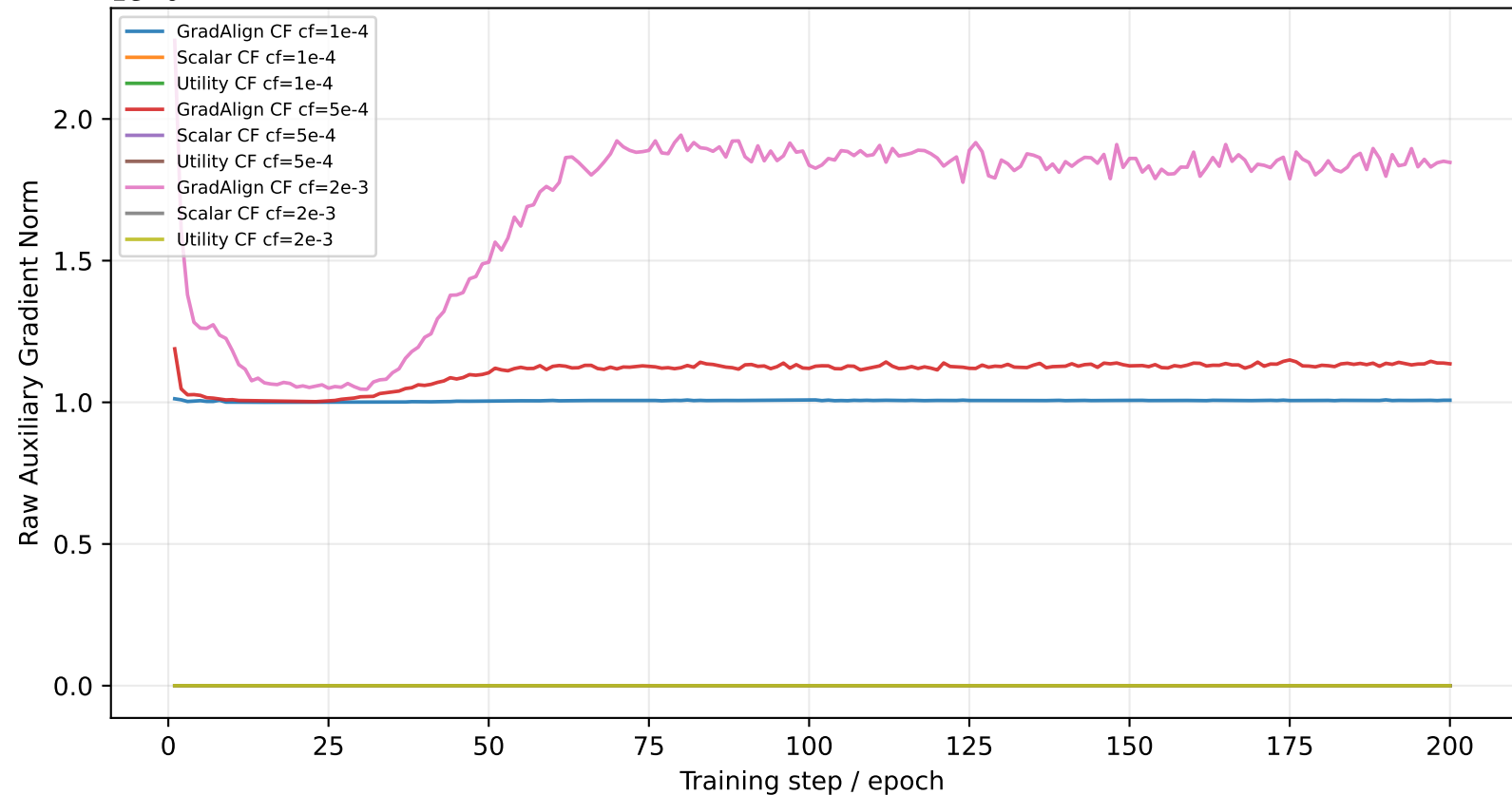
1e-6 Counterfactual Feature-Credit Guidance Diagnostic: Raw Auxiliary Gradient Norm
