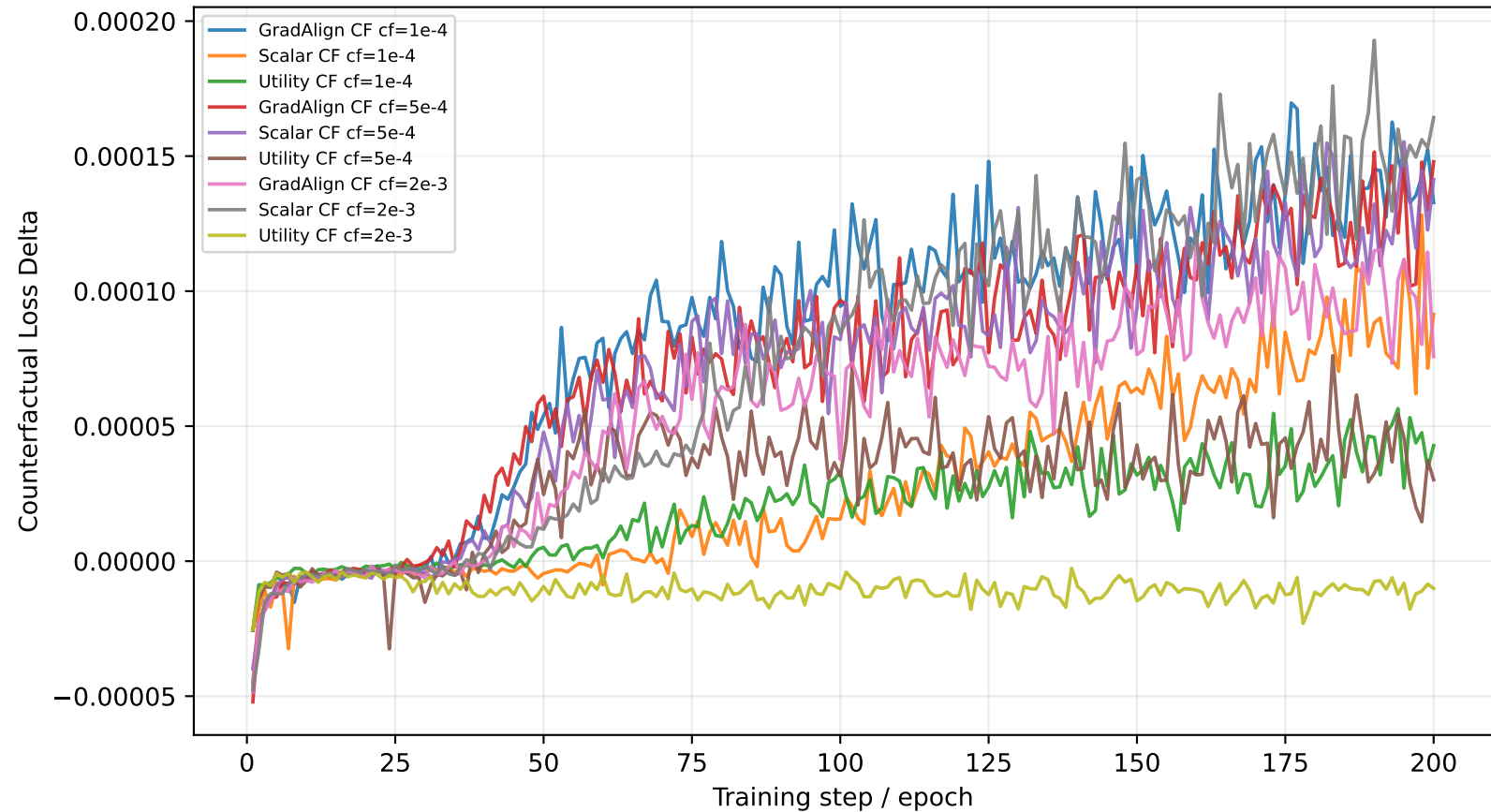
Counterfactual Feature-Credit Guidance Diagnostic: Counterfactual Loss Delta
