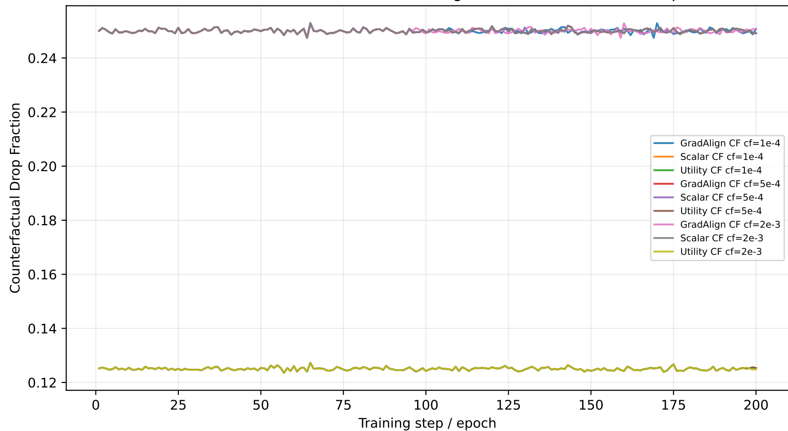
Counterfactual Feature-Credit Guidance Diagnostic: Counterfactual Drop Fraction
