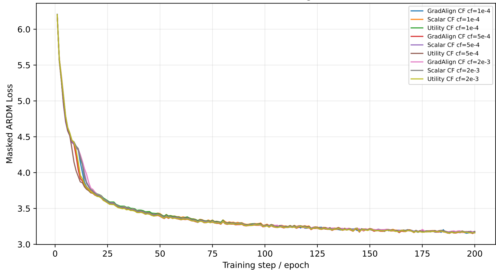
Counterfactual Feature-Credit Guidance Diagnostic: Masked ARDM Loss
