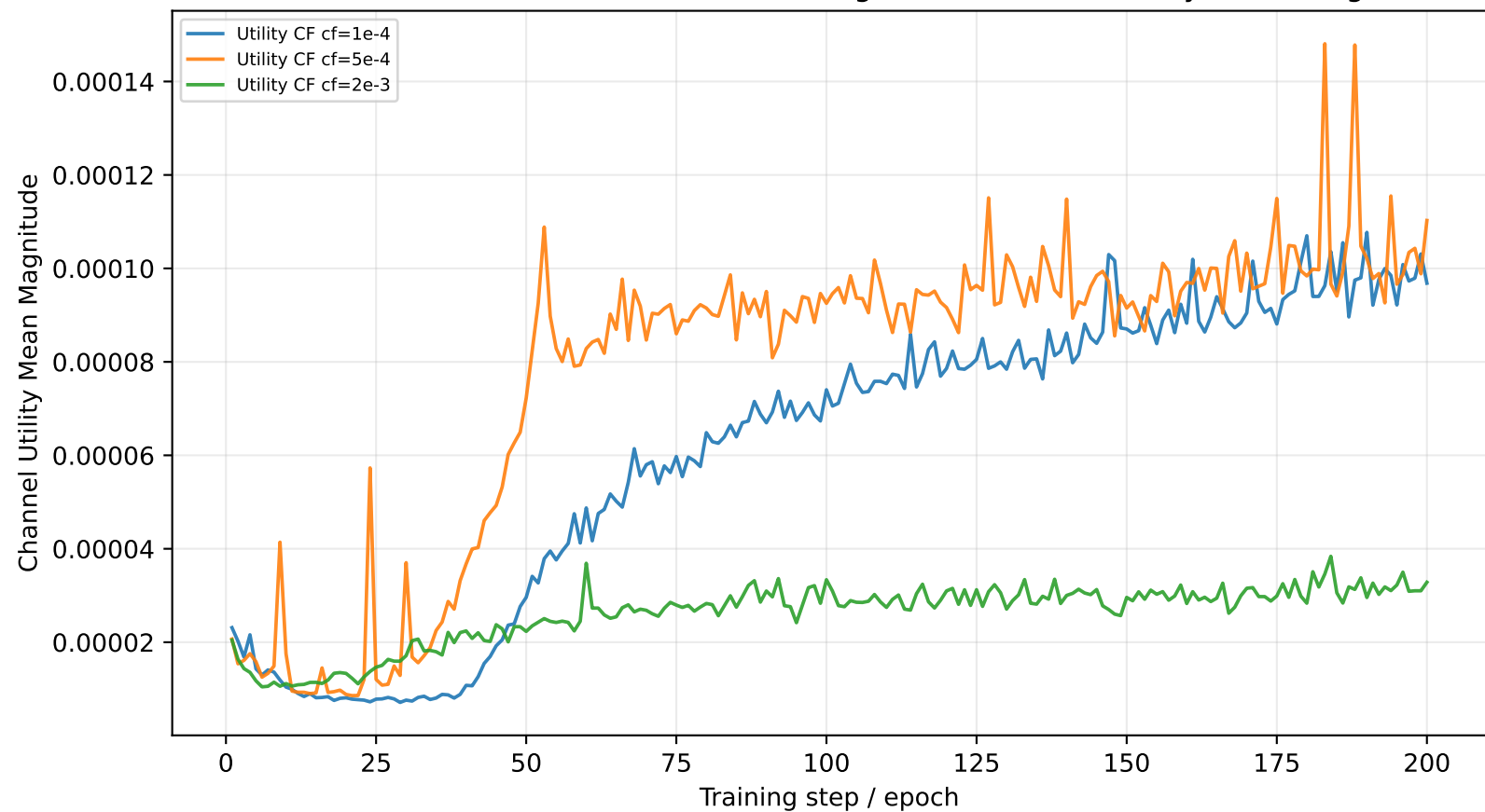
Counterfactual Feature-Credit Guidance Diagnostic: Channel Utility Mean Magnitude
