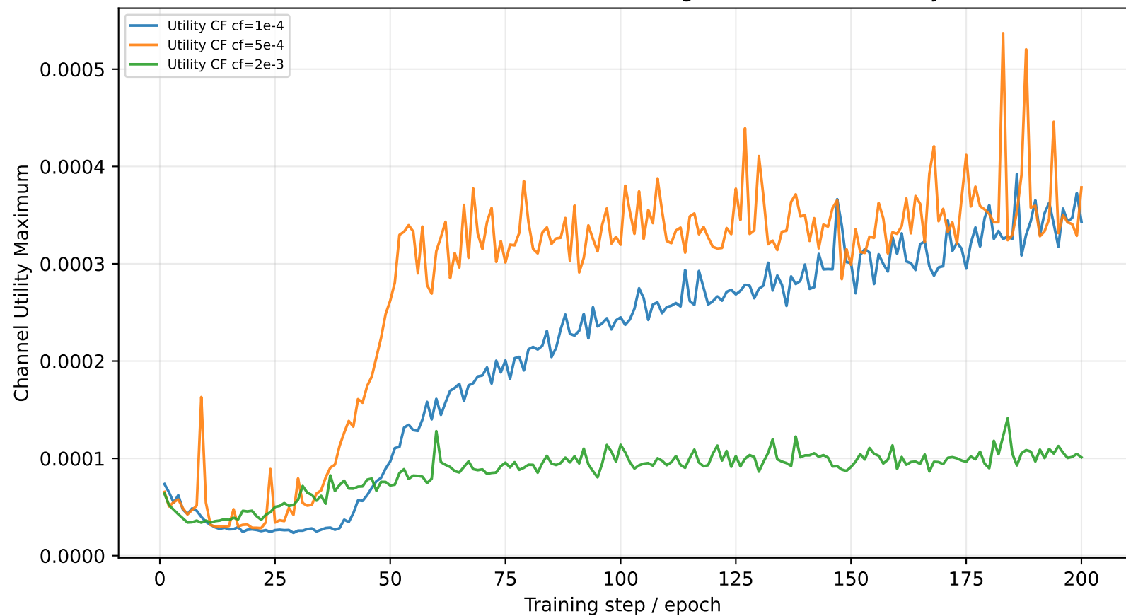
Counterfactual Feature-Credit Guidance Diagnostic: Channel Utility Maximum
