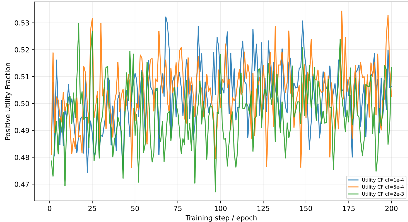
Counterfactual Feature-Credit Guidance Diagnostic: Positive Utility Fraction
