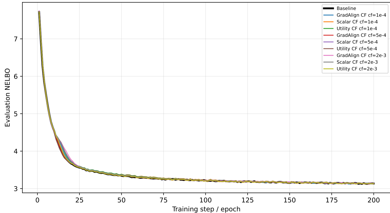
Counterfactual Feature-Credit Guidance: Evaluation NELBO
