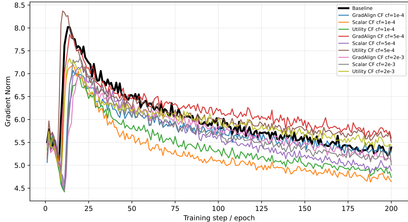
Counterfactual Feature-Credit Guidance: Gradient Norm
