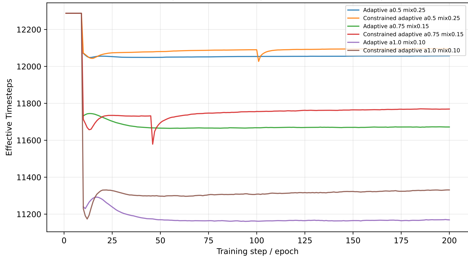
Scheduling-Based ARDM Diagnostic: Effective Timesteps
