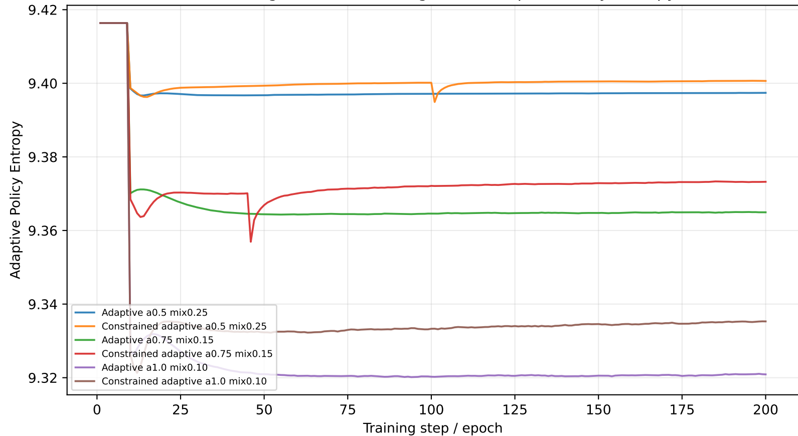
Scheduling-Based ARDM Diagnostic: Adaptive Policy Entropy
