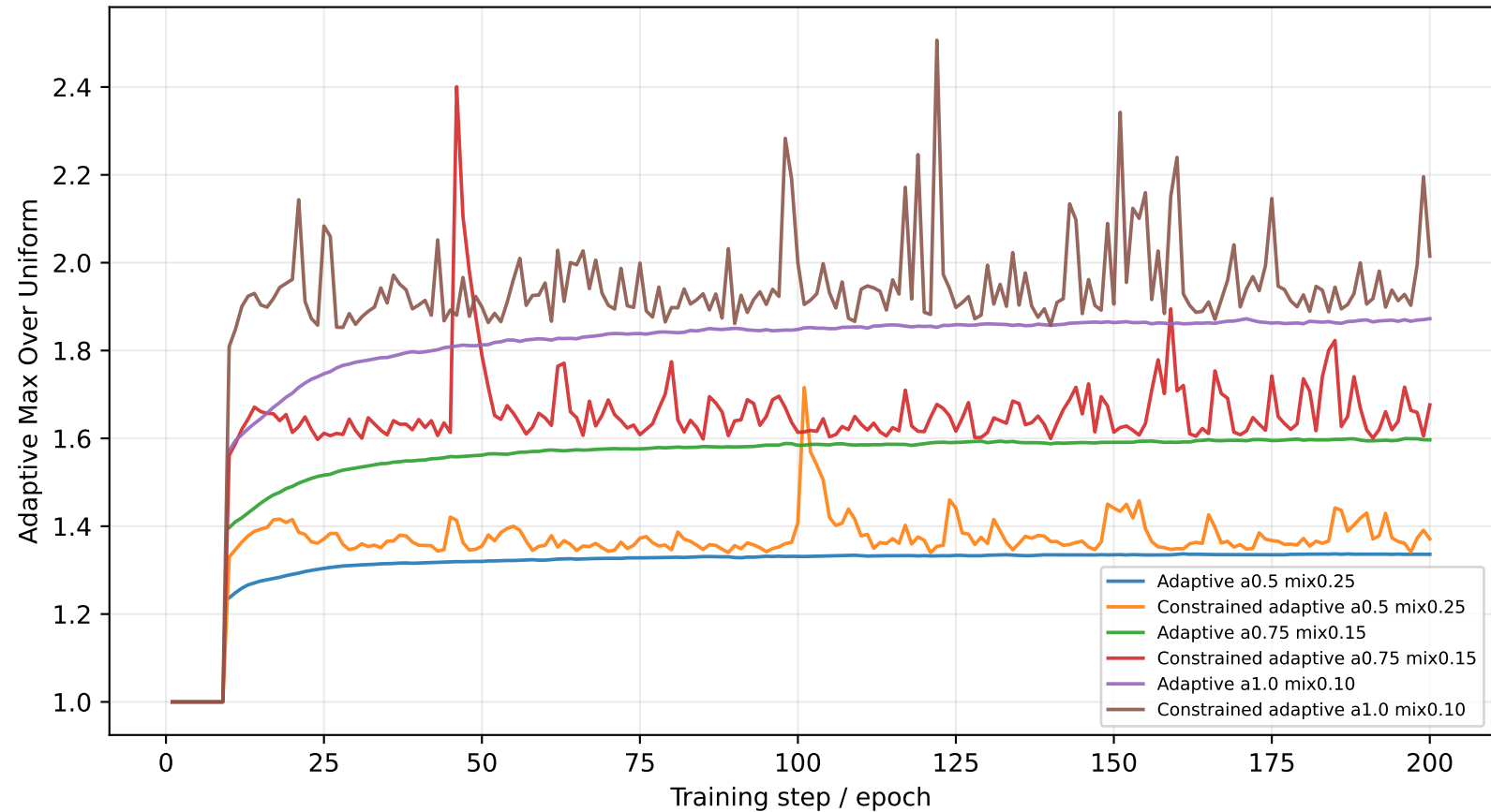
Scheduling-Based ARDM Diagnostic: Adaptive Max Over Uniform
