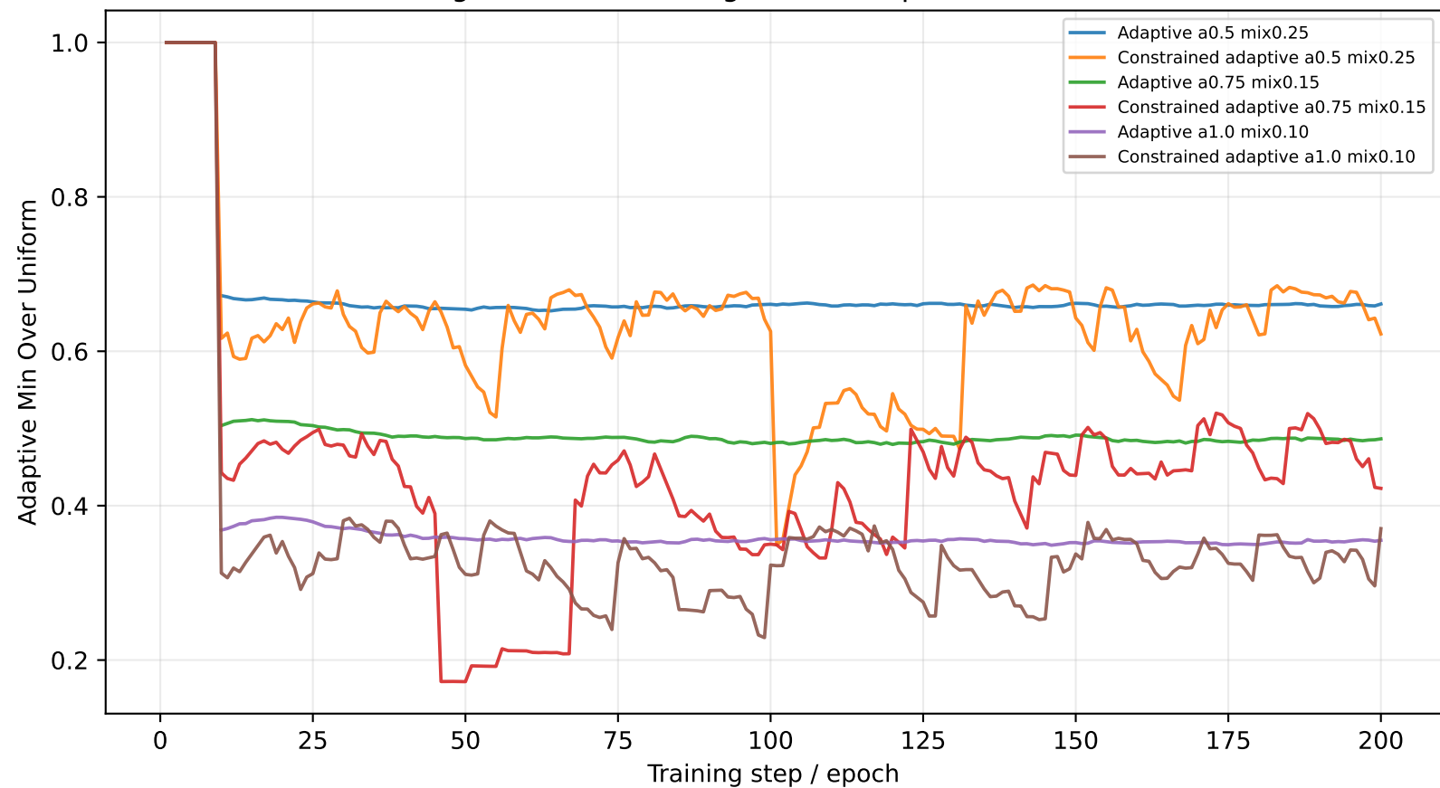
Scheduling-Based ARDM Diagnostic: Adaptive Min Over Uniform
