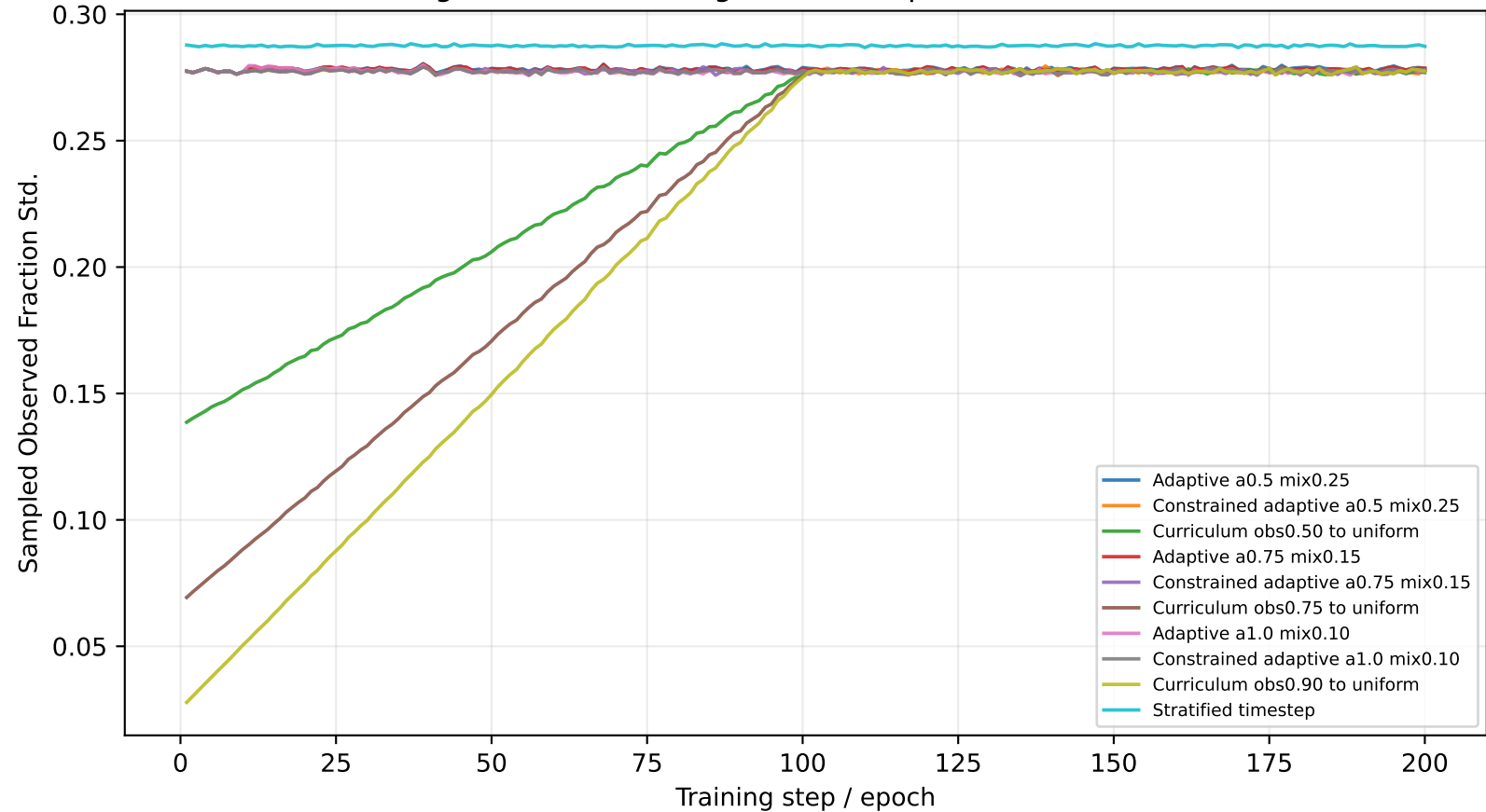
Scheduling-Based ARDM Diagnostic: Sampled Observed Fraction Std.
