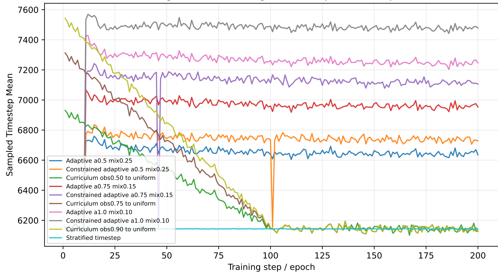
Scheduling-Based ARDM Diagnostic: Sampled Timestep Mean
