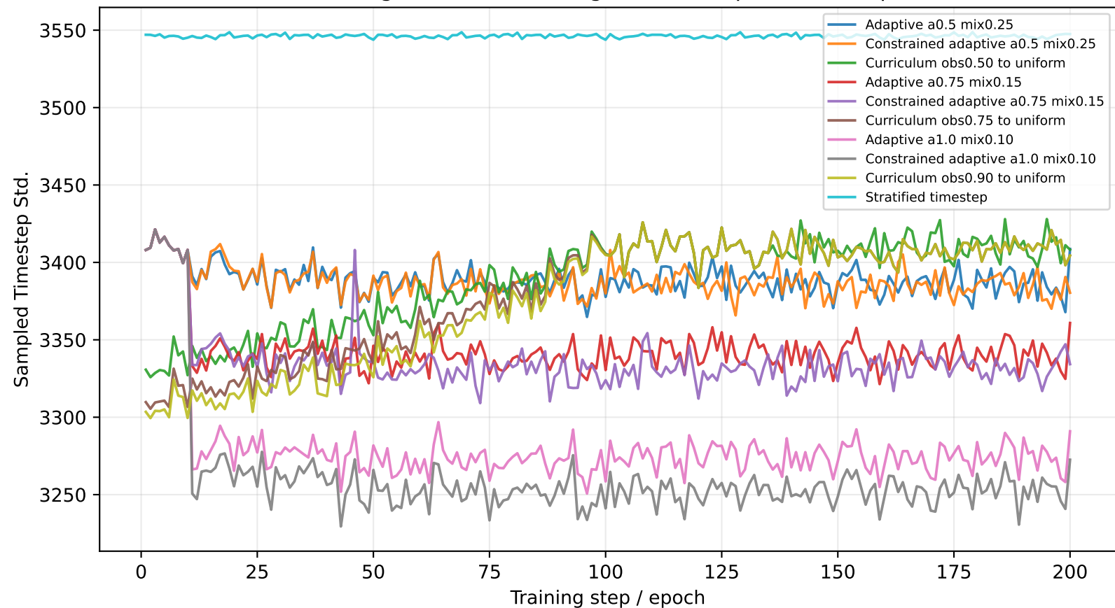
Scheduling-Based ARDM Diagnostic: Sampled Timestep Std.
