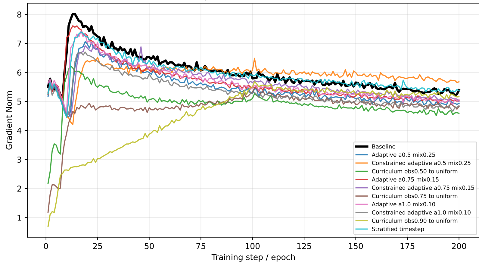
Scheduling-Based ARDM: Gradient Norm
