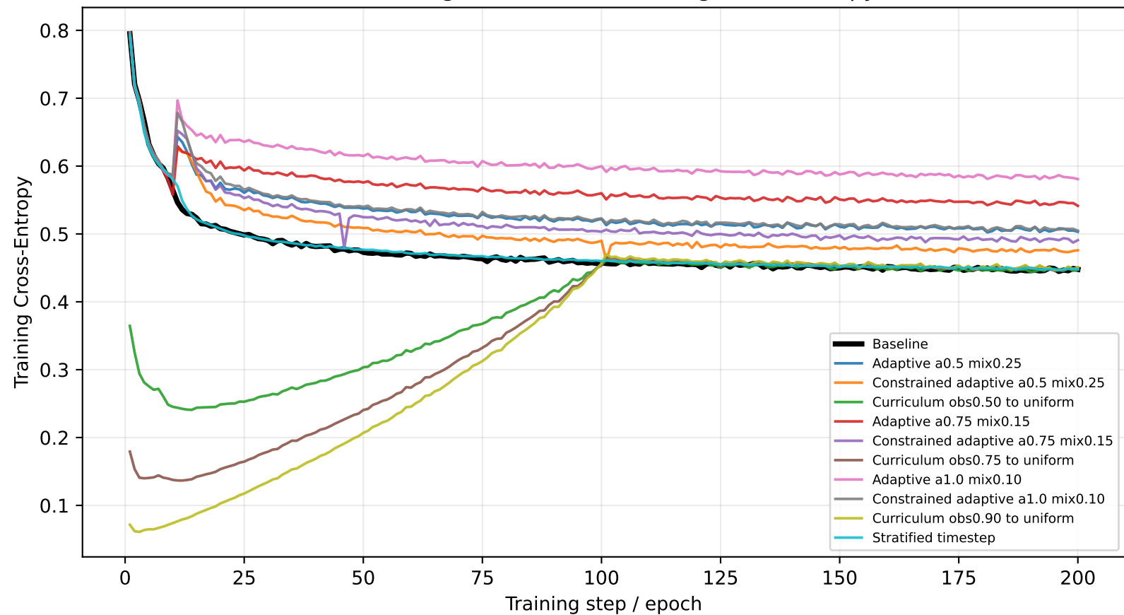
Scheduling-Based ARDM: Training Cross-Entropy
