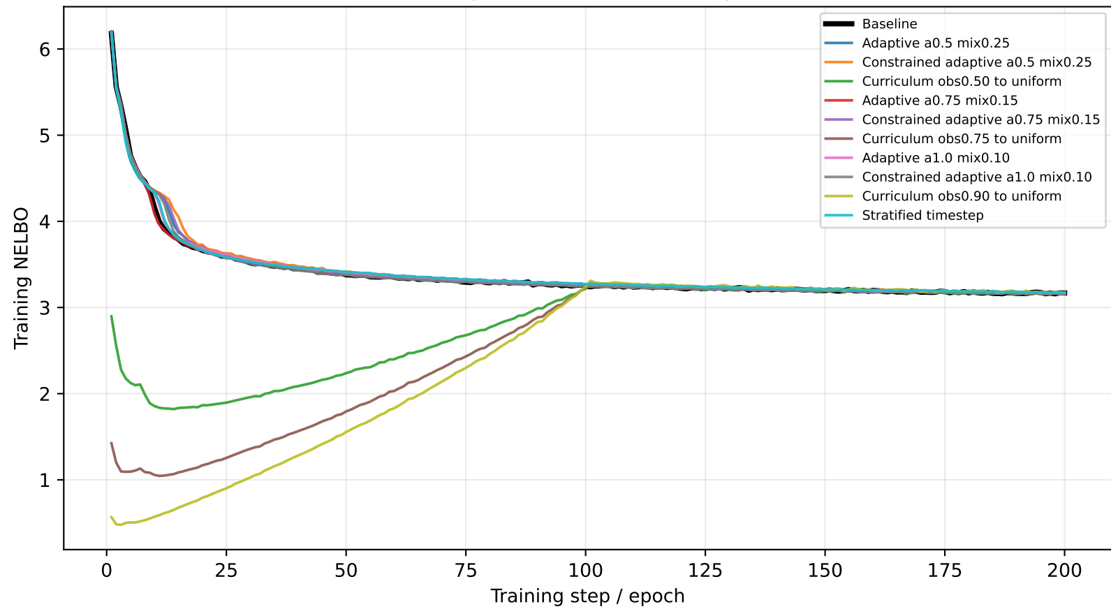
Scheduling-Based ARDM: Training NELBO
