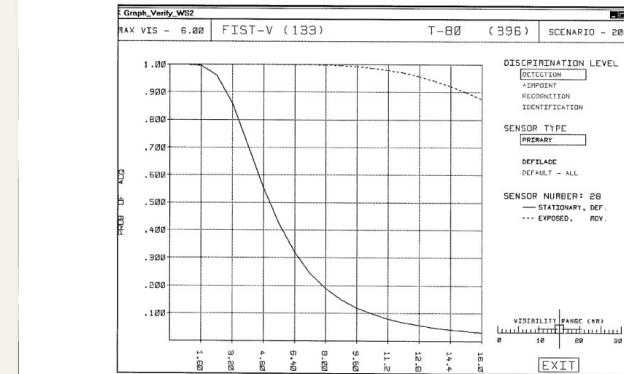
Figure 1. Probability of detection curve versus range (km) for a FistV w/ thermal sights vs. a stationary (solid line) T80.
