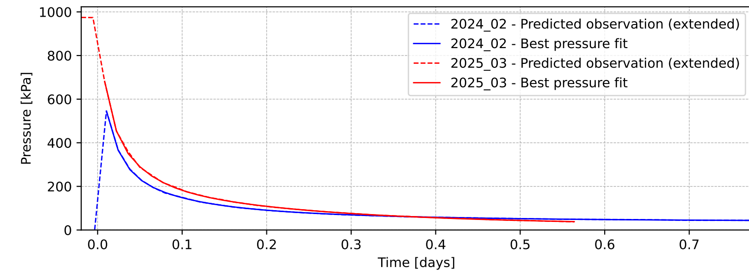
L5-49DL_2 - 2024_02 vs 2025_03 comparison
