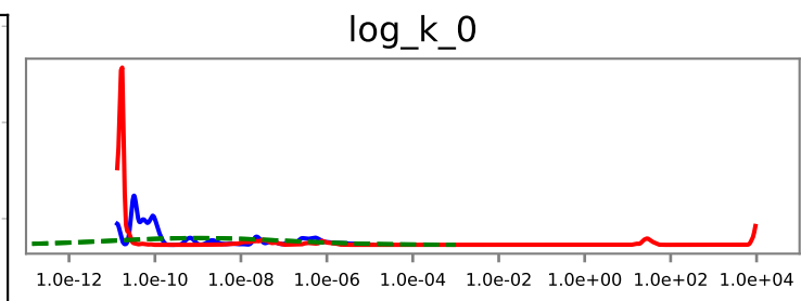
L5-49DL_2 - 2024_02 vs 2025_03 comparison
