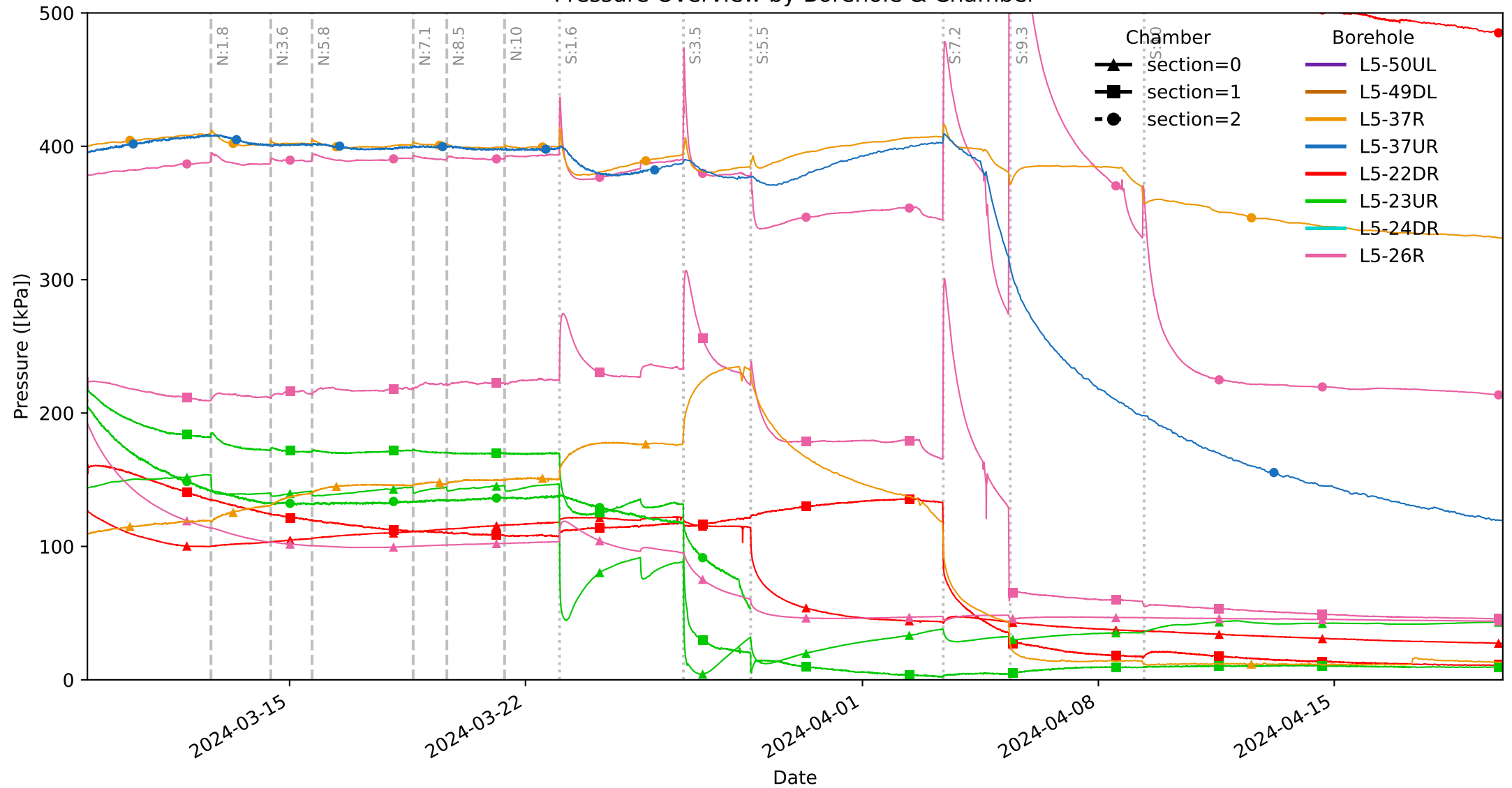
Pressure Overview by Borehole & Chamber
