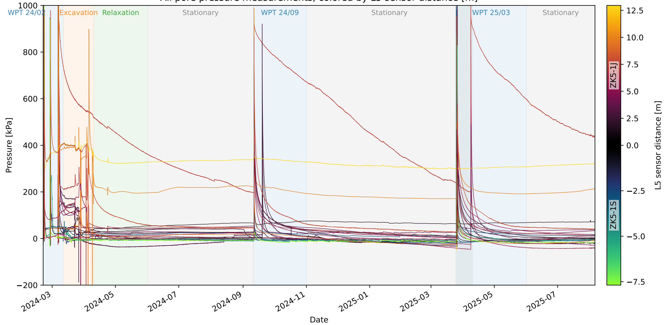
All pore pressure measurements, colored by L5 sensor distance [m]
