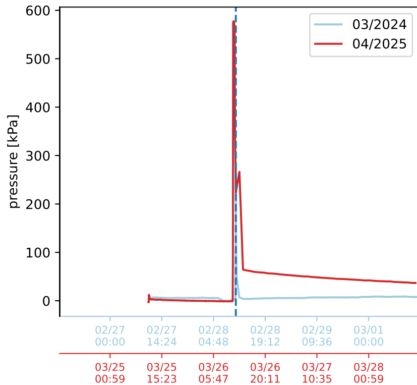
WPT - borehole 37UR section 1
