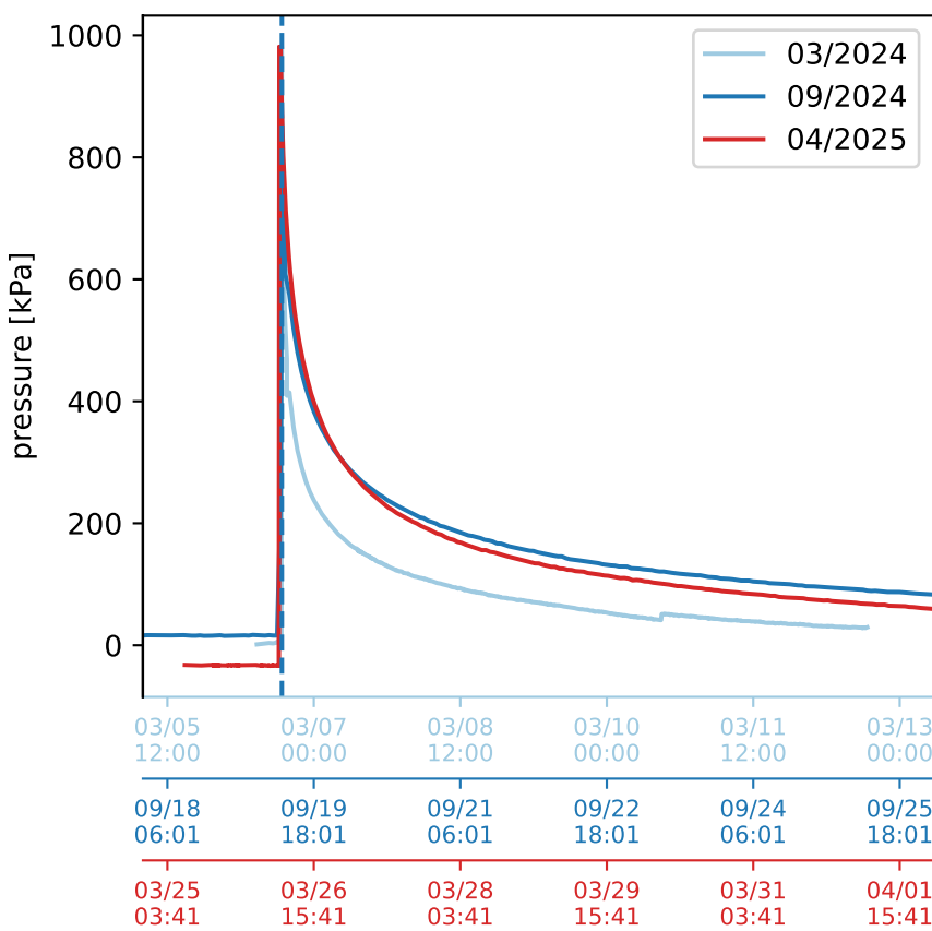
WPT - borehole 24DR section 1
