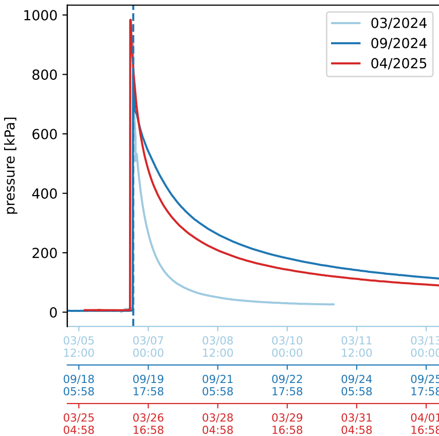
WPT - borehole 24DR section 0
