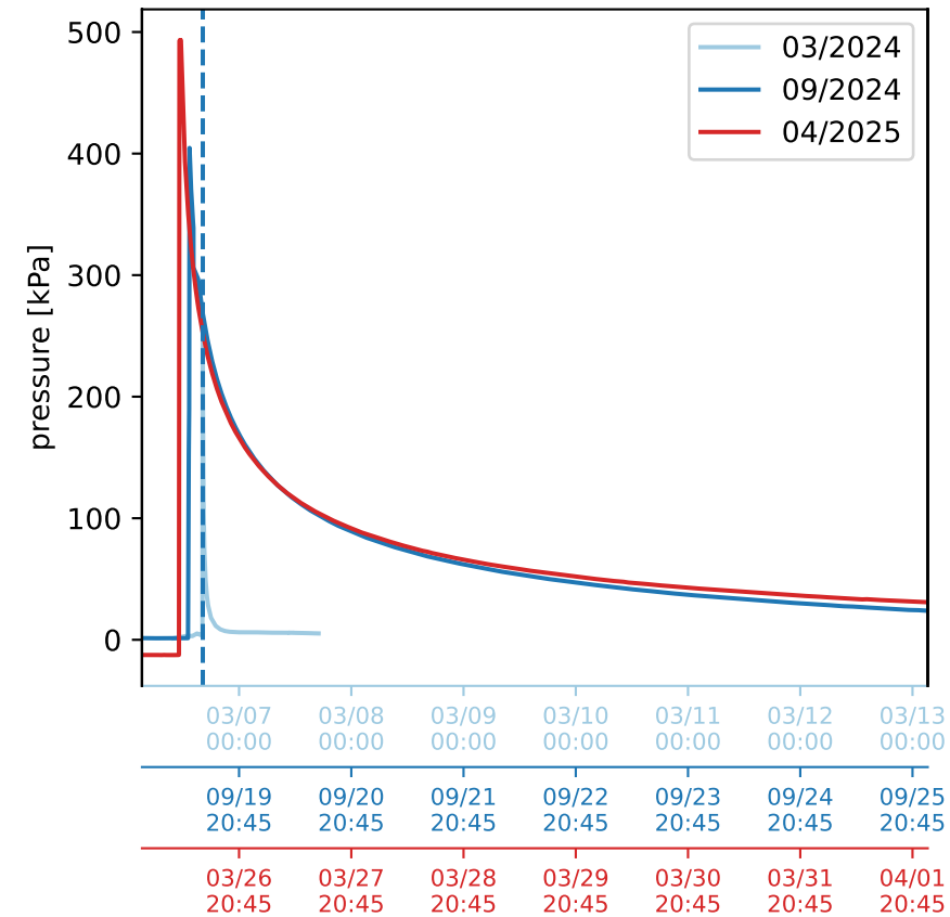
WPT - borehole 24DR section 0
