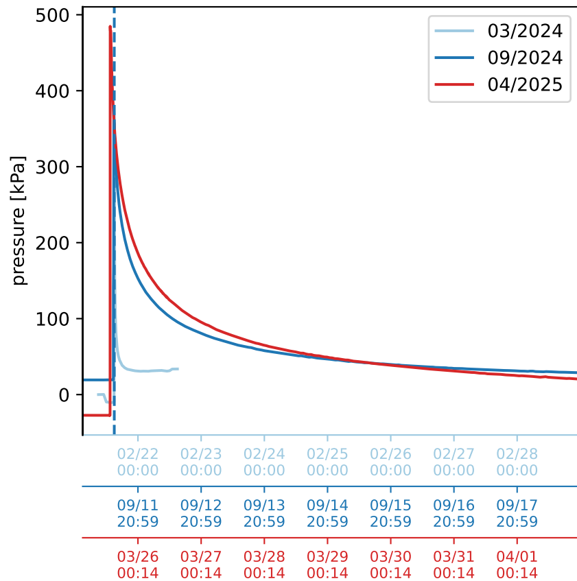
WPT - borehole 37UR section 0
