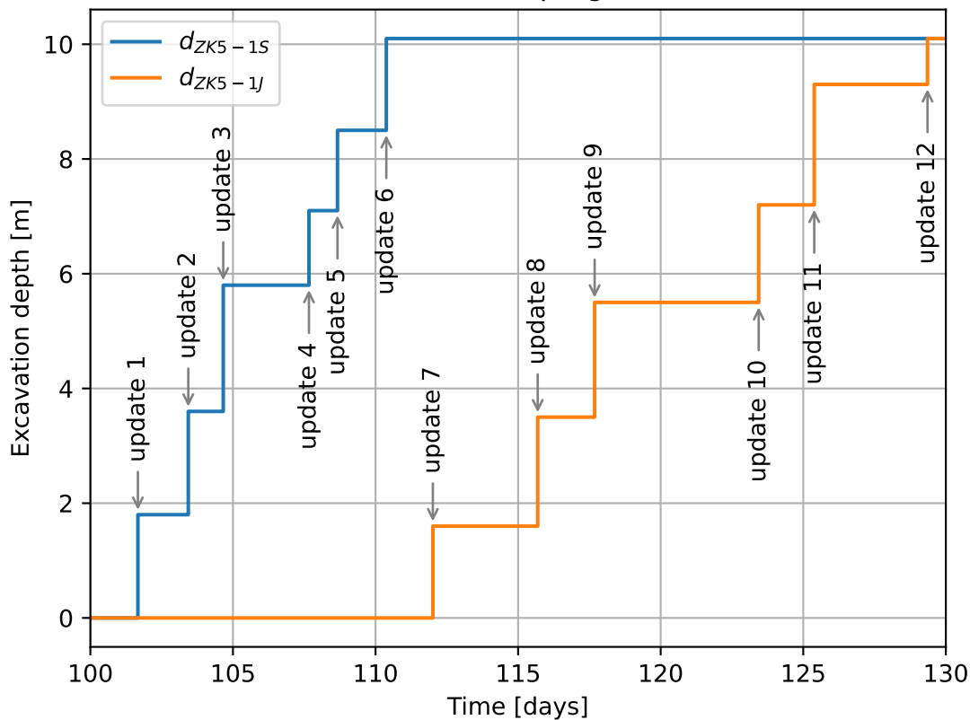
Excavation progress
