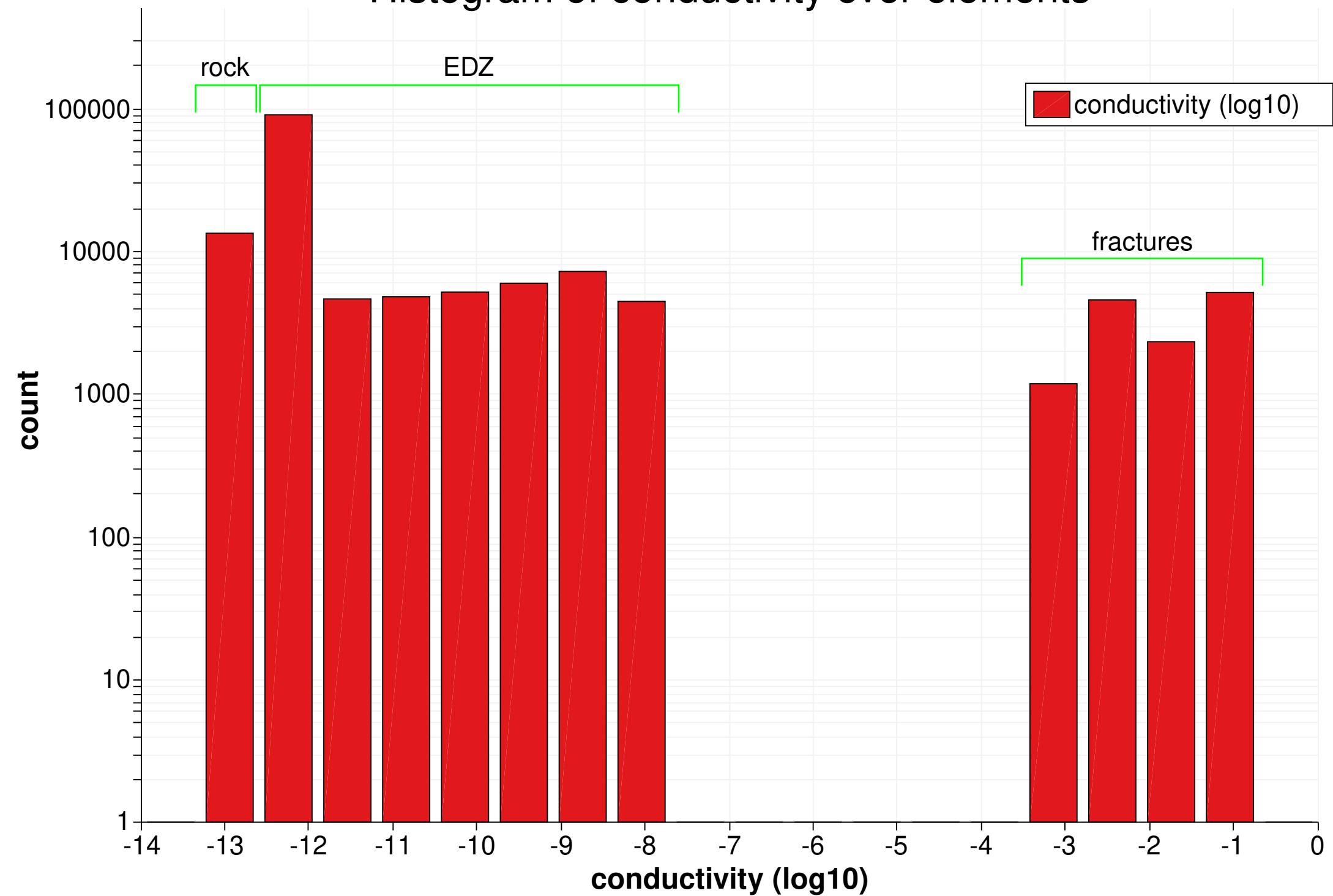
Histogram of conductivity over elements
