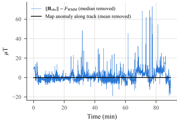
(b) Magnetic: observed intensity varies by microtesla
