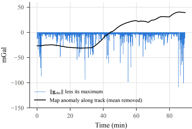
(a) Gravity: norm pinned at 9.806650 \text{ m/s}^2 (63% within 1 mGal)
