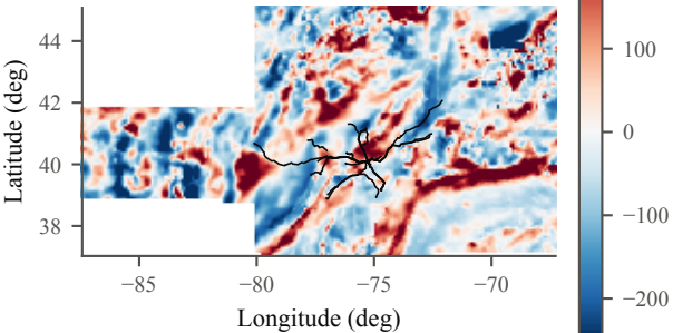
(a) WDMAM magnetic anomaly, 3 arc-min
