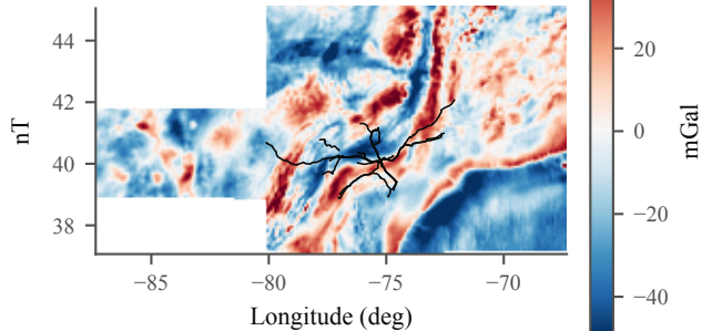
(b) IGPP free-air gravity anomaly, 1 arc-min
