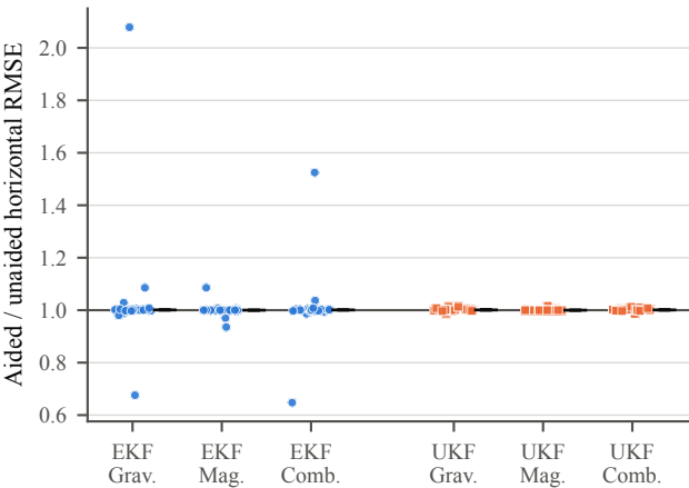
(a) Smartphone observations
