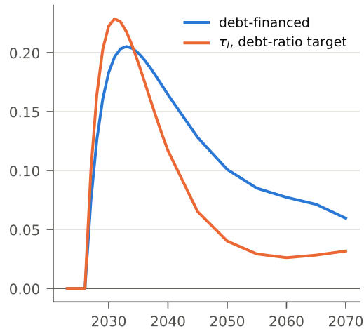
Gini, wealth, change in points
