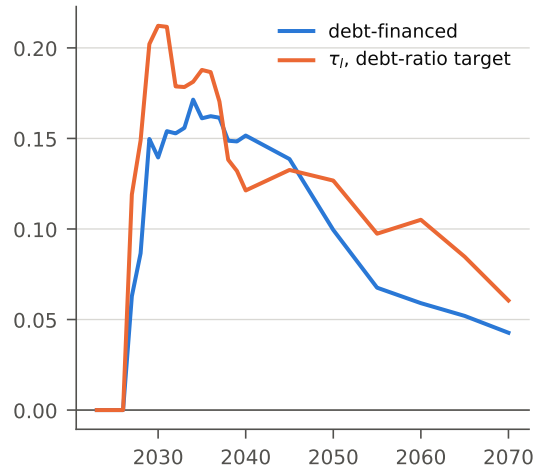
Top-10% wealth share, change in points
