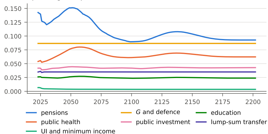
Spending / output
