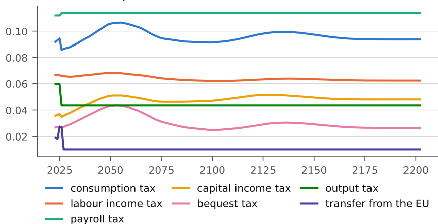
Revenue / output
