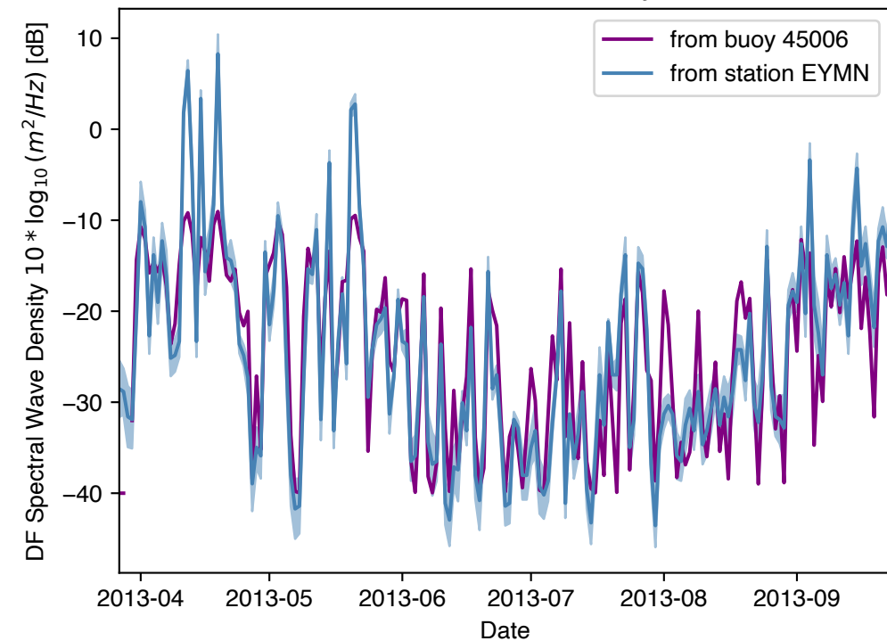
Lake Wave State - Wave Buoy 45006
