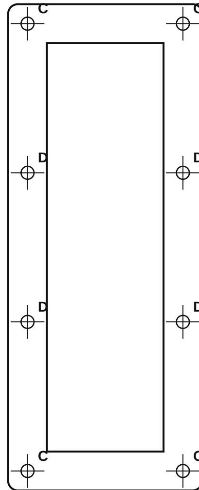
frame (weldment) — 2.500" × 6.250"
