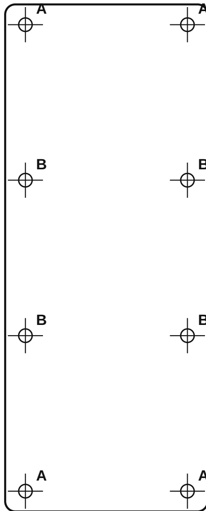
middle — 2.500" × 6.250"
