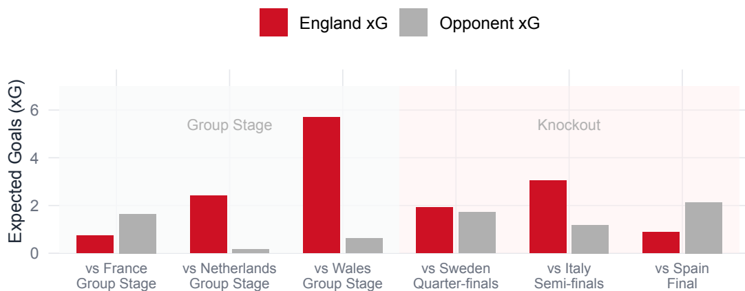
Figure 4: Match-by-match xG for England across the tournament. Red bars show England xG, grey bars show opponent xG. England's group stage total is heavily influenced by the 6-1 win against Wales.
