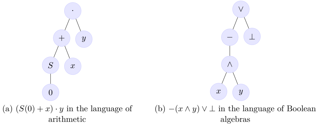
Figure 6.1: Term tree
