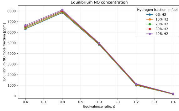
(a) Equilibrium NO.
