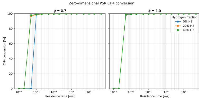
Figure 10: Ideal PSR CH 4 conversion versus residence time at T_{\text{in}} = 1000 K, p = 10 atm, \phi = 0.7 and 1.0. Conversion is shown only as a finite-rate stirred-reactor trend; it does not include mixing, geometry, wall heat loss or turbine-combustor residence time distributions.
