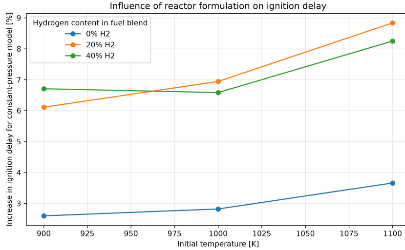
Figure 6: Ignition delay at \phi = 1.0 and p = 10 atm: constant-volume versus constant-pressure reactor for T_0 = 900, 1000 and 1100 K, and hydrogen fractions of 0, 20 and 40 mol %.
