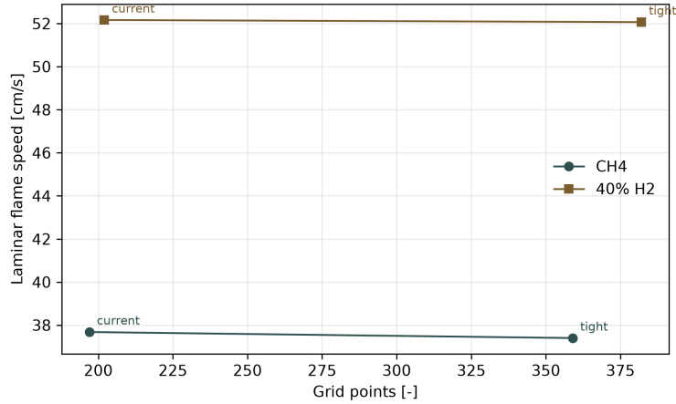
Figure 8: Diagnostic comparison of current and tight FreeFlame refinement settings. The check is a grid-refinement consistency check for two representative cases, not a validation against measurements.
