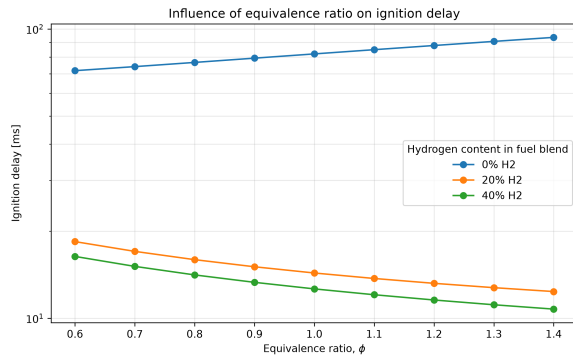
(a) Ignition delay.
