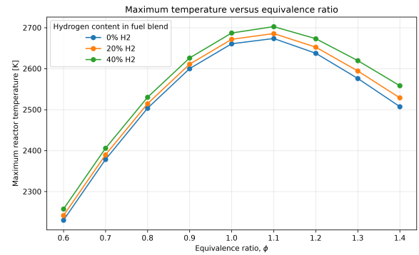
(b) Maximum temperature.
