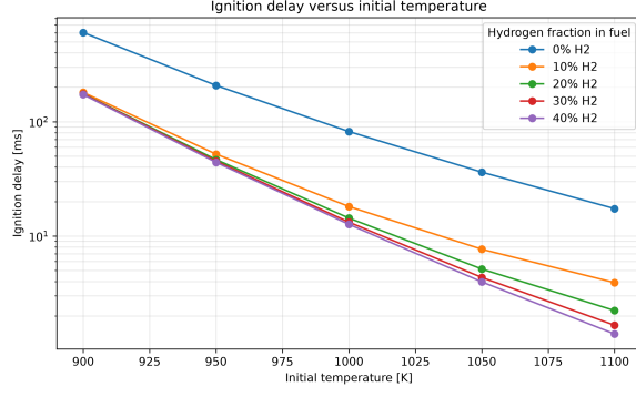
(a) Versus initial temperature at \phi = 1.0 and p = 10 atm.
