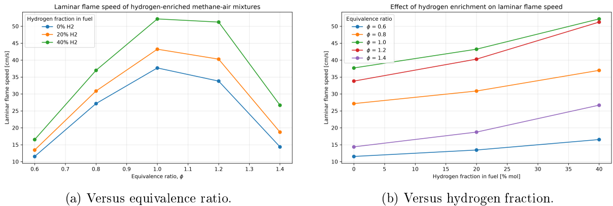
Figure 7: Laminar flame speed of hydrogen-enriched methane–air flames.
