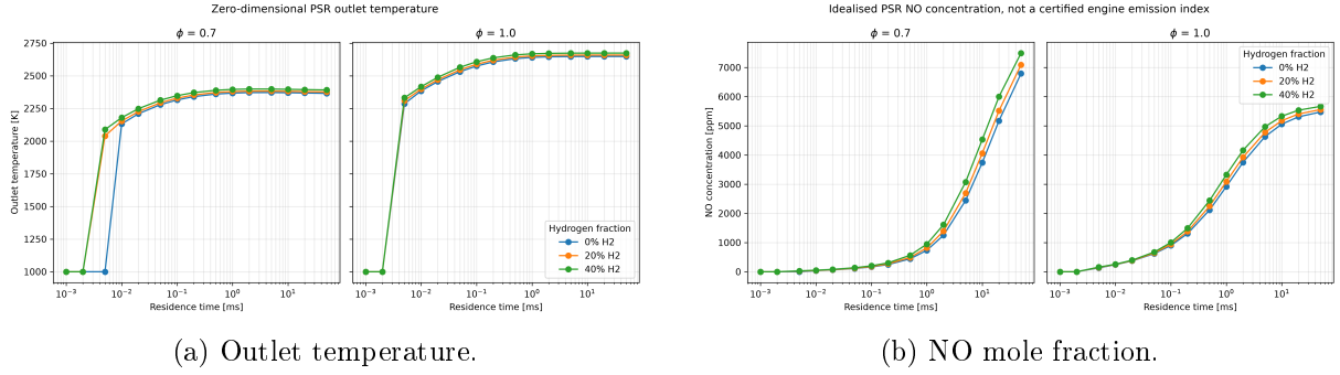
Figure 9: PSR behaviour versus residence time; the drop at short residence time marks a stability-transition bracket on the tested grid. Inlet conditions are T_{\text{in}} = 1000 K, p = 10 atm, with \phi = 0.7 and 1.0.
