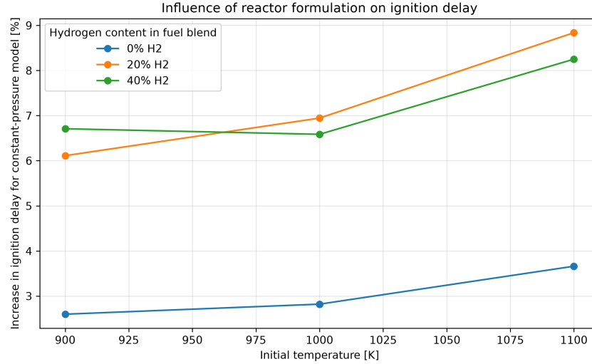
Figure 6: Ignition delay at \phi = 1.0 and p = 10\text{ atm} : constant-volume versus constant-pressure reactor for T_0 = 900, 1000 and 1100\text{ K} , and hydrogen fractions of 0, 20 and 40 mol %.
