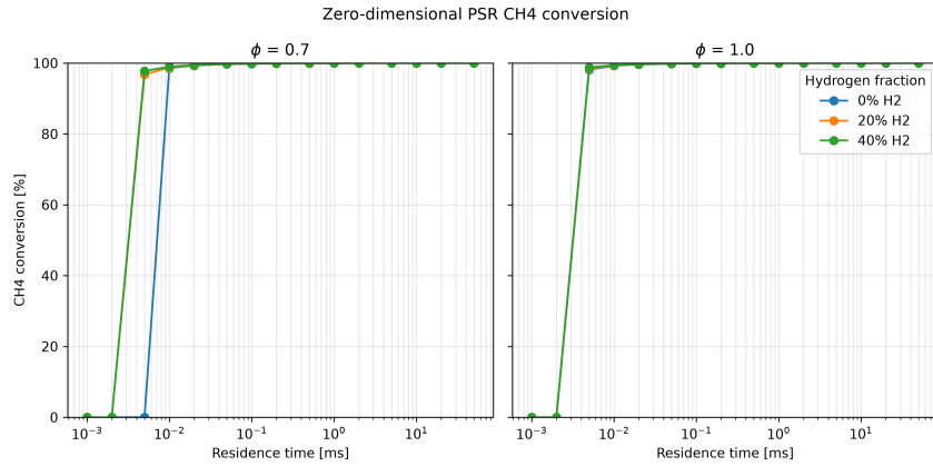
Figure 10: Ideal PSR \text{CH}_4 conversion versus residence time at T_{in} = 1000 K, p = 10 atm, \phi = 0.7 and 1.0. Conversion is shown only as a finite-rate stirred-reactor trend; it does not include mixing, geometry, wall heat loss or turbine-combustor residence time distributions.
