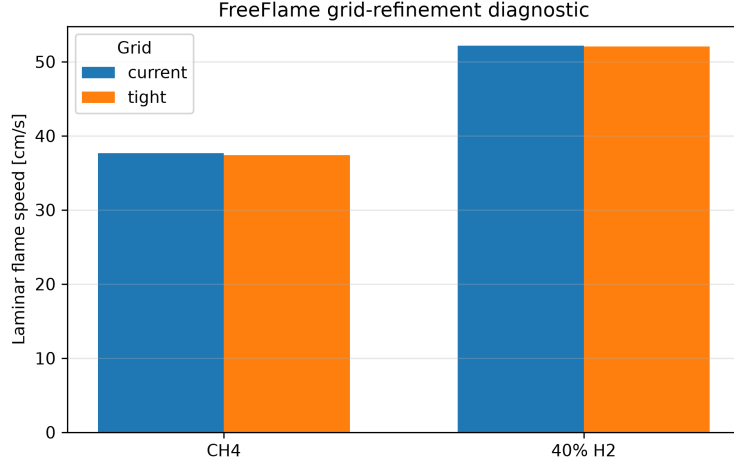
Figure 8: Diagnostic comparison of current and tight FreeFlame refinement settings. The check is a grid-refinement consistency check for two representative cases, not a validation against measurements.
