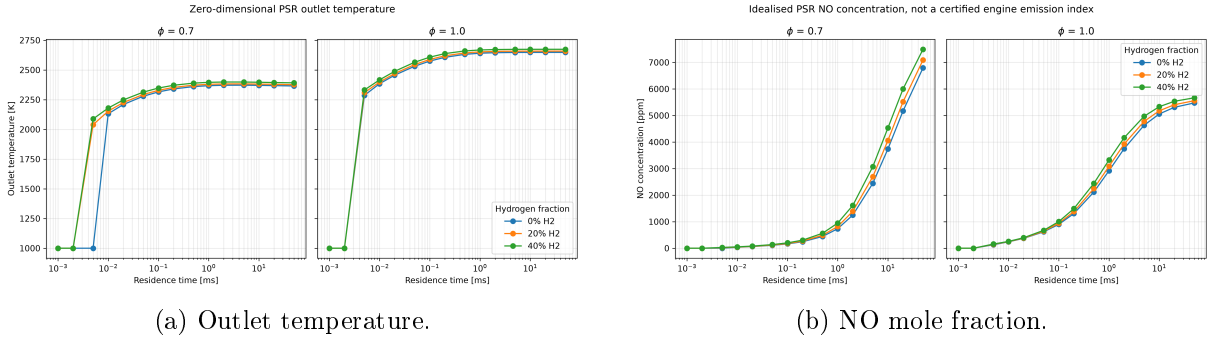
Figure 9: PSR behaviour versus residence time; the drop at short residence time marks a stability-transition bracket on the tested grid. Inlet conditions are T_{in} = 1000 K, p = 10 atm, with \phi = 0.7 and 1.0.
