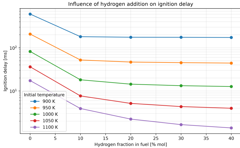
Figure 4: Constant-pressure ignition delay versus hydrogen fraction at \phi = 1.0 , p = 10 atm and T_0 = 900 –1100 K. The logarithmic axis highlights that the strongest enrichment effect occurs between pure methane and the first hydrogen-containing blend in this grid.
