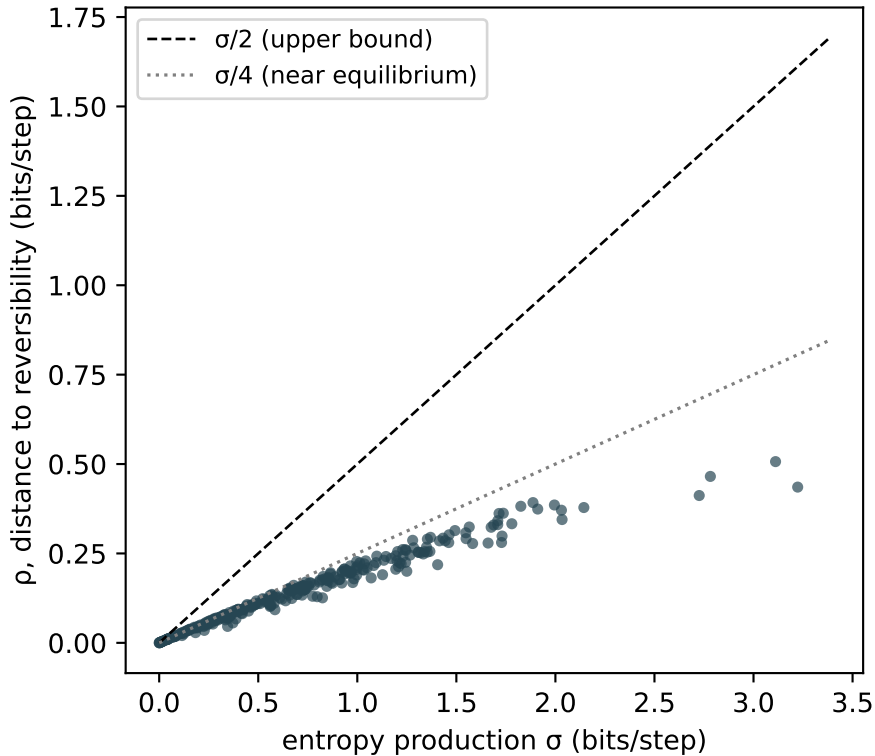
\rho vs \sigma for 300 random chains
