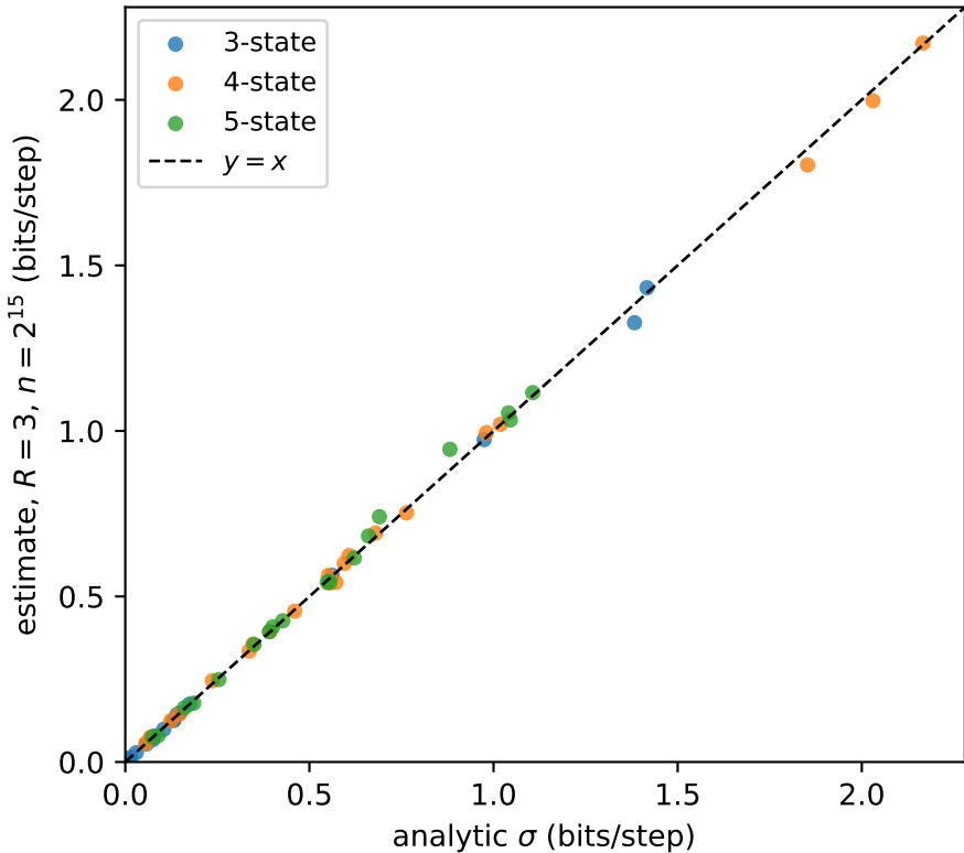
Calibration across 60 random chains
