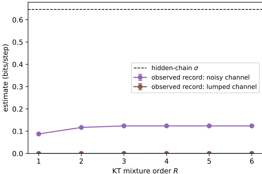
Observed irreversibility of a hidden ring ( n = 2^{17} , 3 seeds)
