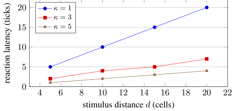
Figure 2: The internal light cone: reaction latency to a one-tick stimulus reveal. Fit over all points: latency = 0.99(d/\kappa) + 0.17 , R^2 = 0.999 — information moves through the fields at 1.01 cells per sweep, the theoretical maximum of a radius-1 stencil.
