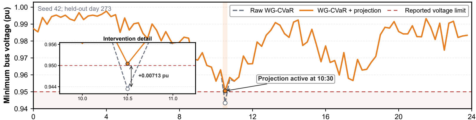
(a) Voltage restoration on the worst confirmed day
