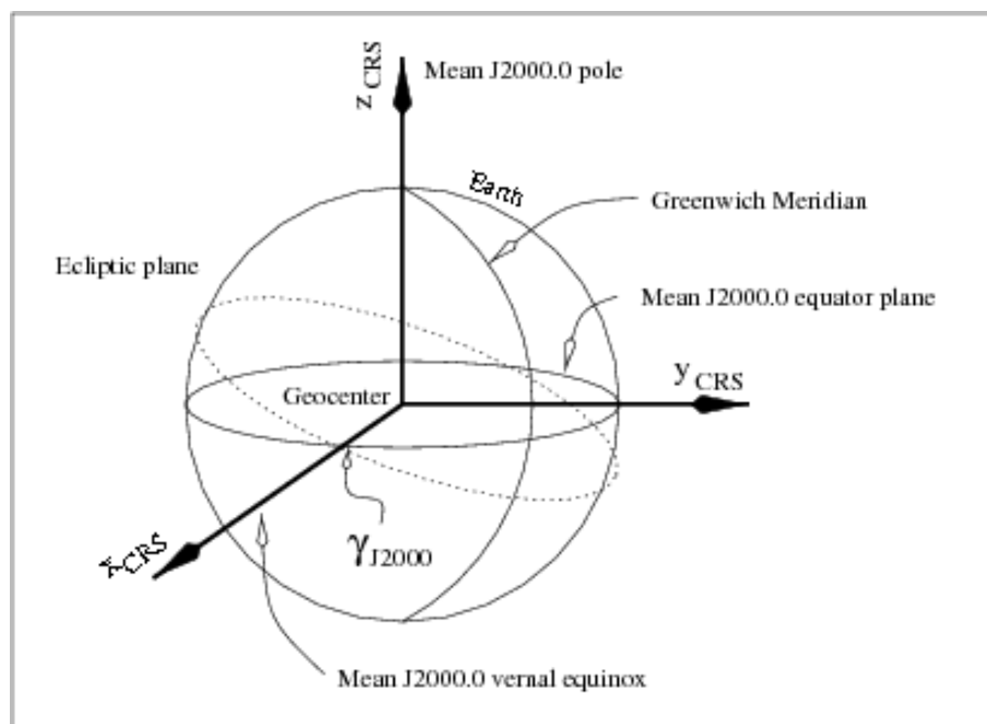
FIGURE 1.1 – Principe du Geocentric Celestial Reference Frame. Source : Navipedia, ESA.
